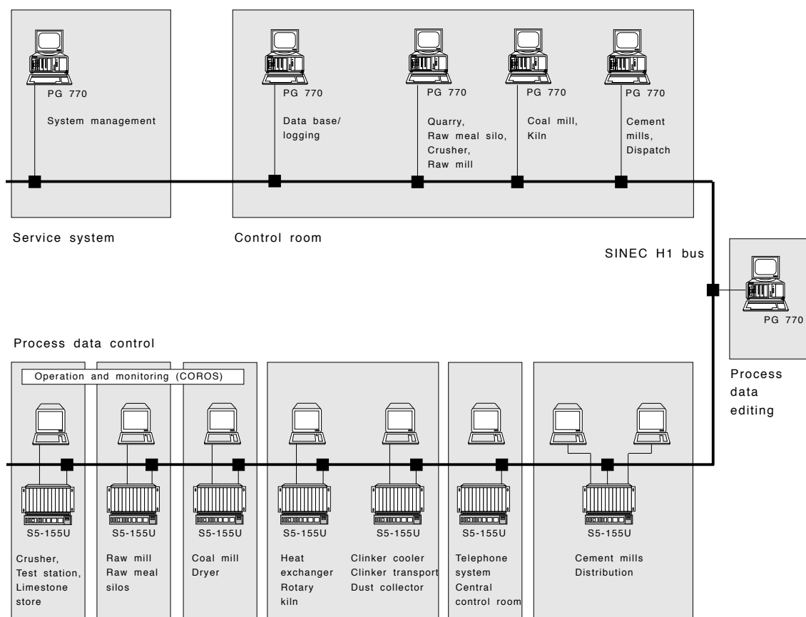
Fig. 1-1 Example of application of the S5-155U with the CPU 948
